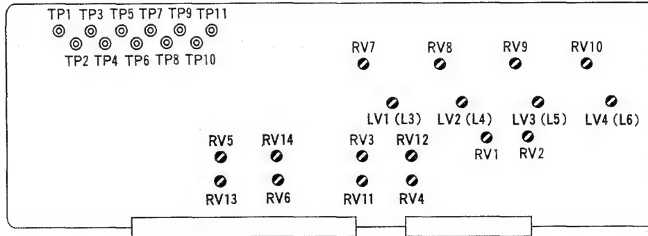
RF-15 board (component side)
